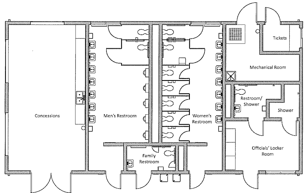
Floor Plan
